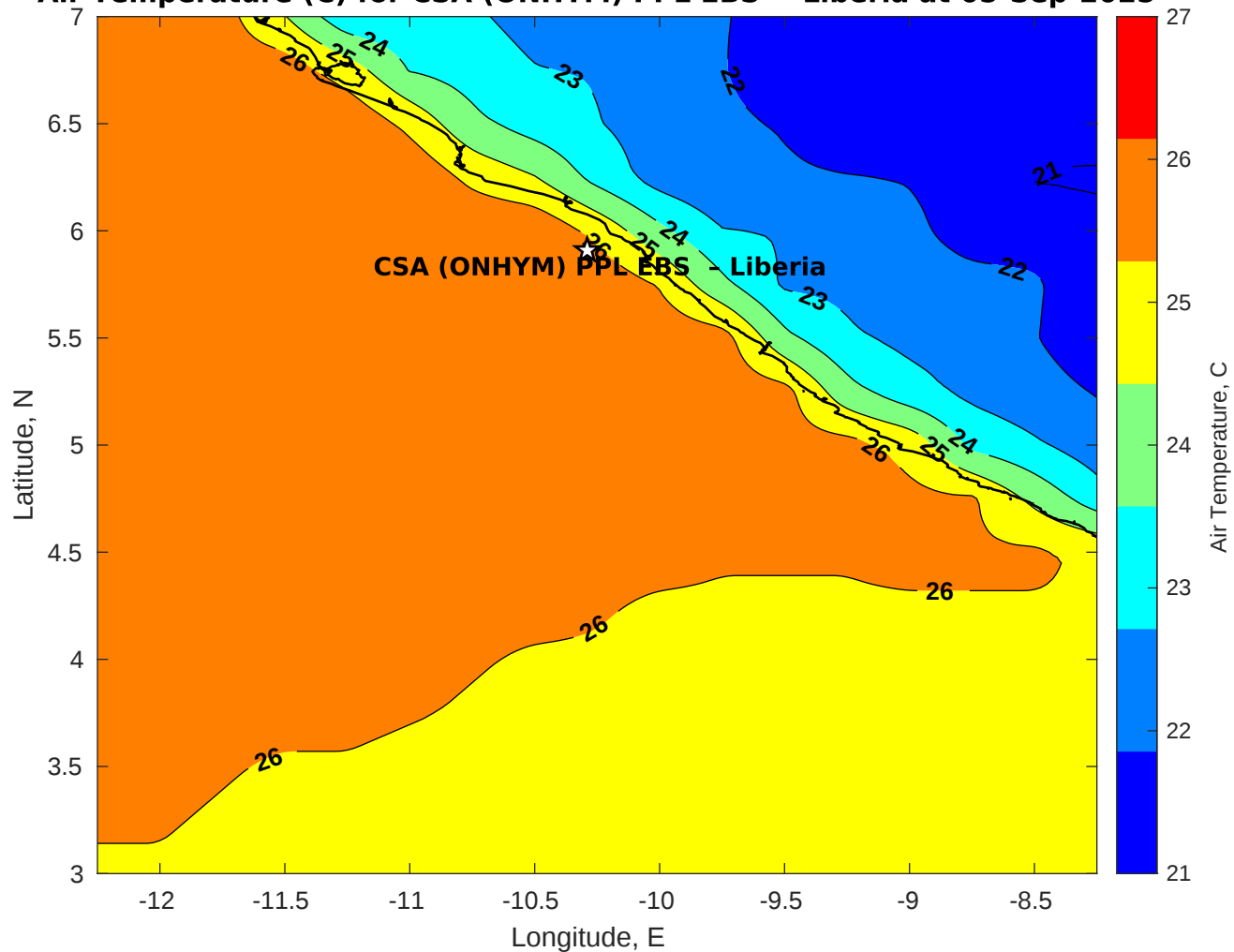
Air Temperature (C) for CSA (ONHYM) PPL EBS - Liberia at 05-Sep-2025
