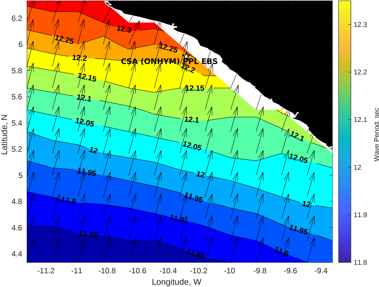
Wave Period (sec) for CSA (ONHYM) PPL EBS - Liberia at 05-Sep-2025 09:00:00
