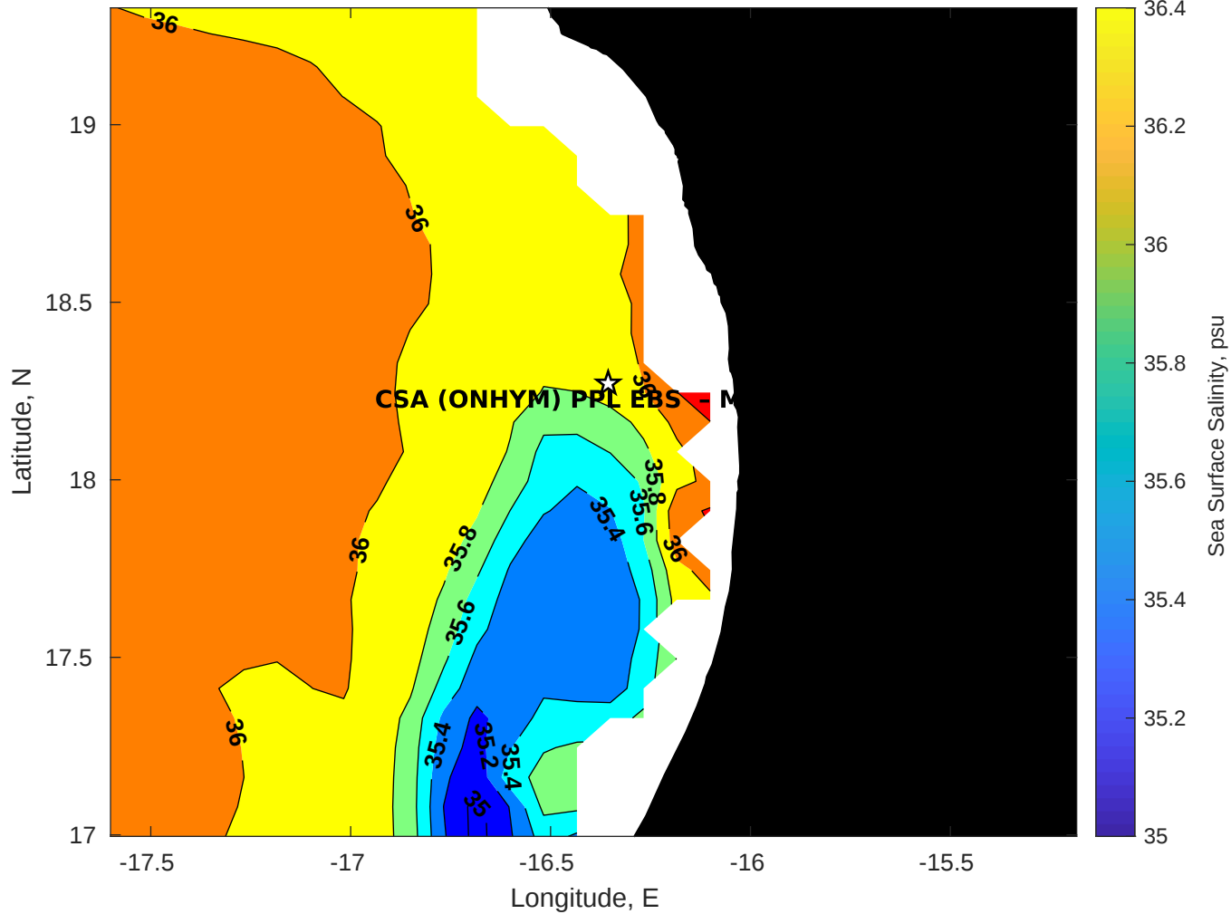
Surface Salinity for CSA (ONHYM) PPL EBS - Mauritania at 04-Sep-2025 00:00:00
