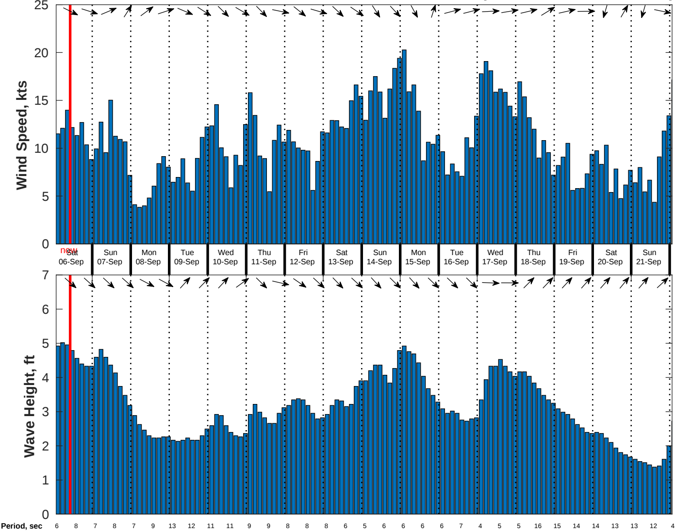
Wind & Wave Forecast for CSA (ONHYM) PPL EBS - Mauritania from 05-Sep-2025 01:00:00 to 21-Sep-2025 01:00:00
