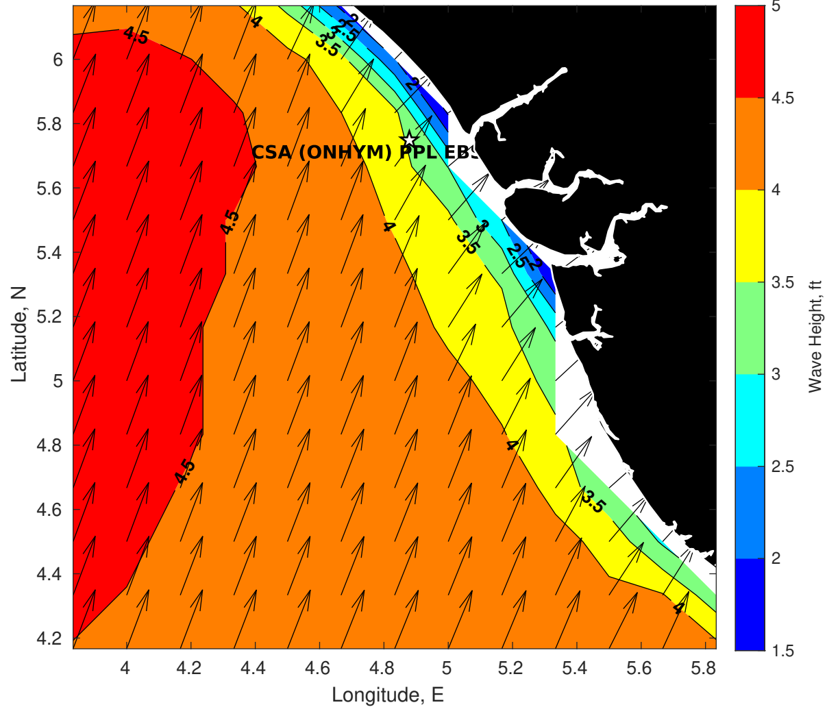
Wave Height (ft) for CSA (ONHYM) PPL EBS - Nigeria at 05-Sep-2025 09:00:00
