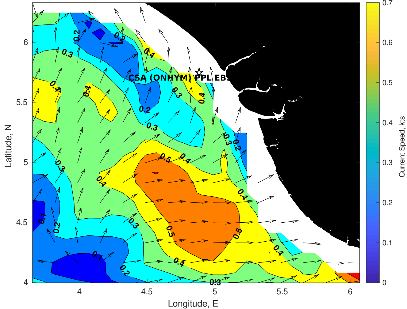
Surface Currents for CSA (ONHYM) PPL EBS - Nigeria at 04-Sep-2025 00:00:00
