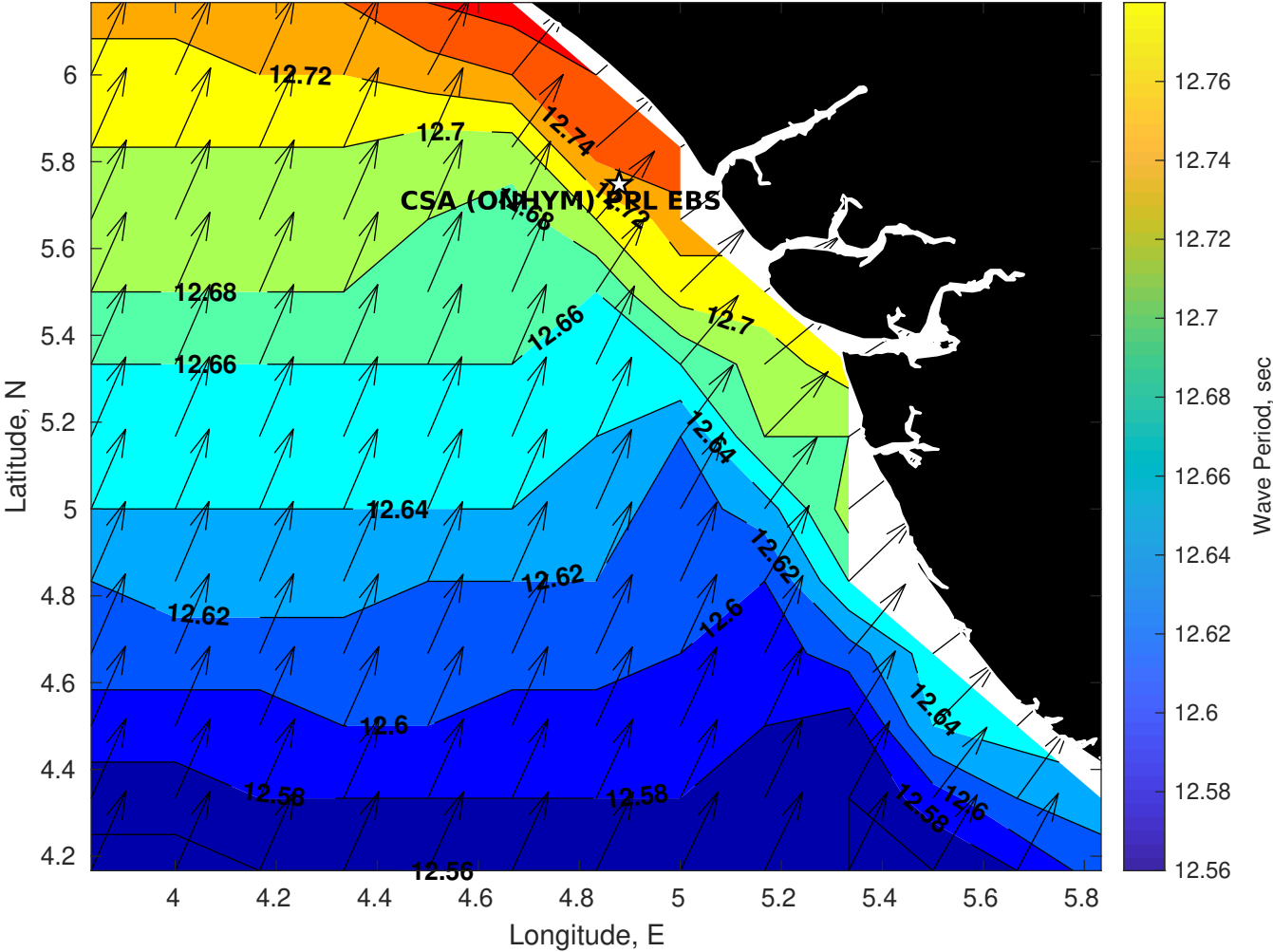
Wave Period (sec) for CSA (ONHYM) PPL EBS - Nigeria at 05-Sep-2025 09:00:00
