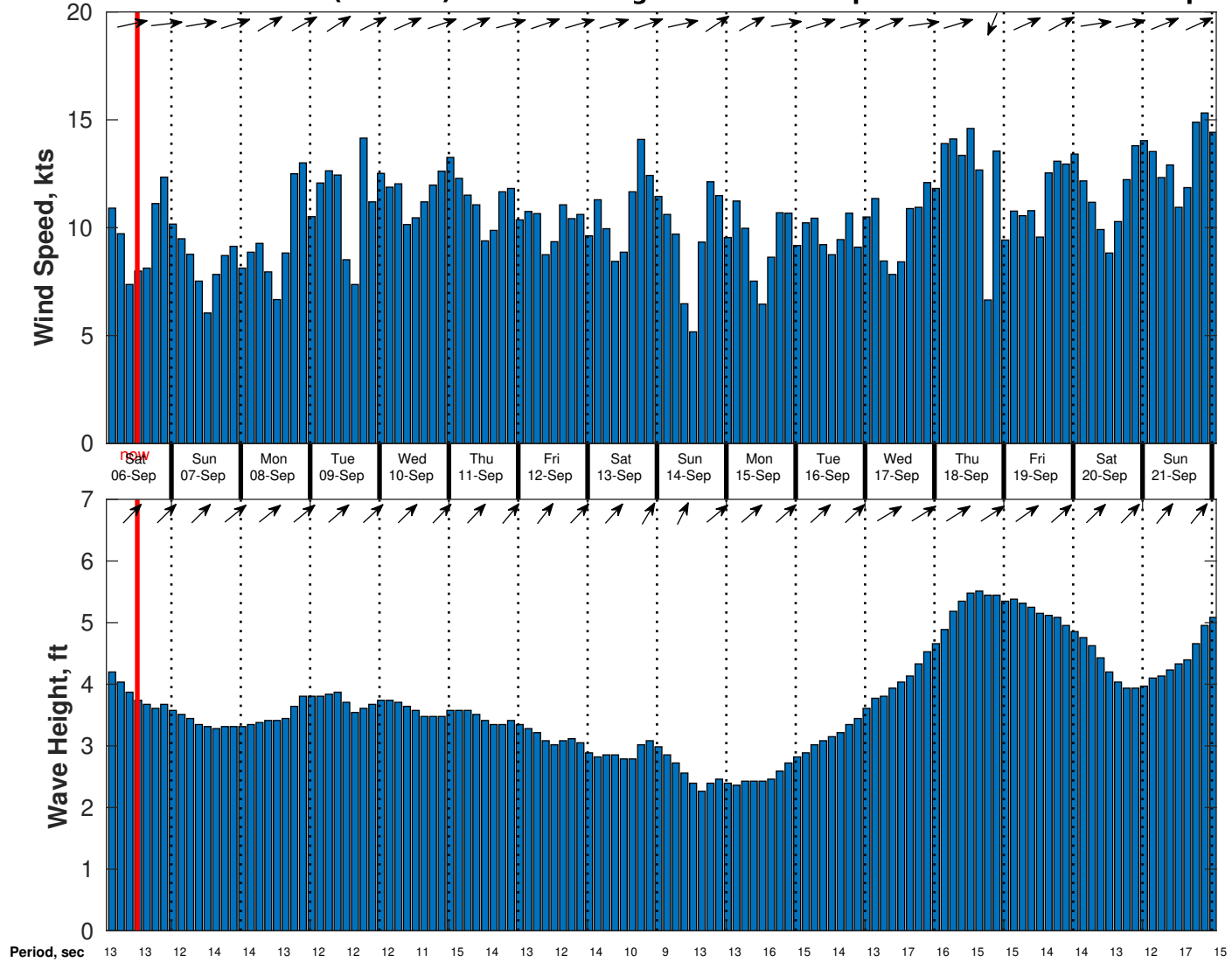
Wind & Wave Forecast for CSA (ONHYM) PPL EBS - Nigeria from 05-Sep-2025 02:00:00 to 21-Sep-2025 02:00:00
