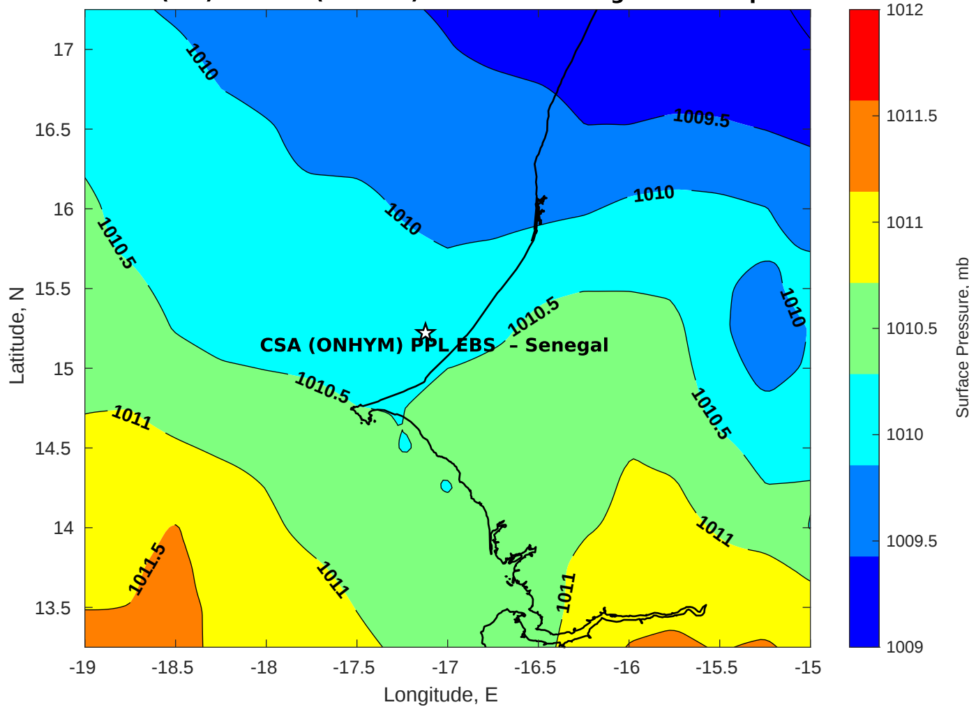
Surface Pressure (mb) for CSA (ONHYM) PPL EBS - Senegal at 06-Sep-2025 00:00:00
