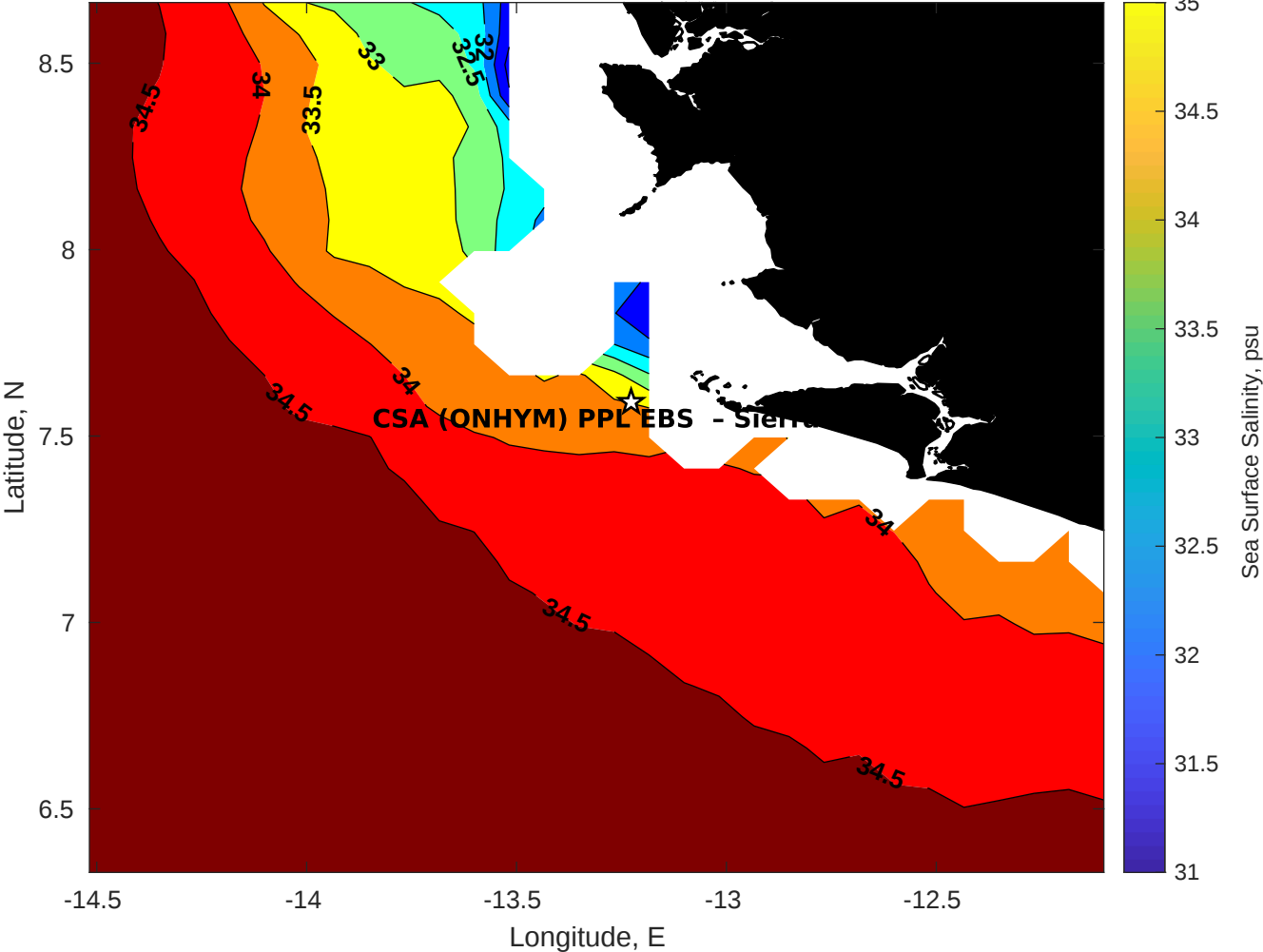
Surface Salinity for CSA (ONHYM) PPL EBS - Sierra Leone at 04-Sep-2025 00:00:00
