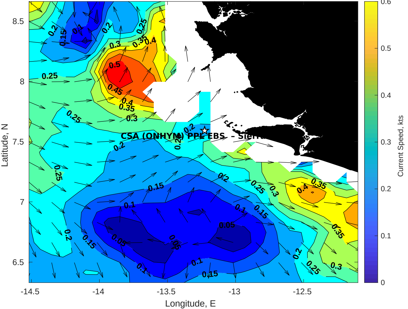
Surface Currents for CSA (ONHYM) PPL EBS - Sierra Leone at 04-Sep-2025 00:00:00
