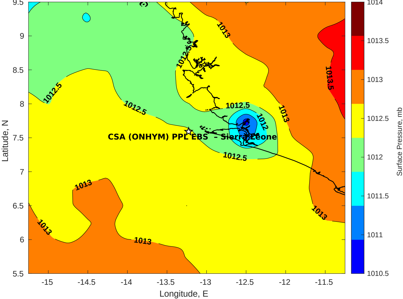
Surface Pressure (mb) for CSA (ONHYM) PPL EBS - Sierra Leone at 05-Sep-2025 00:00:00
