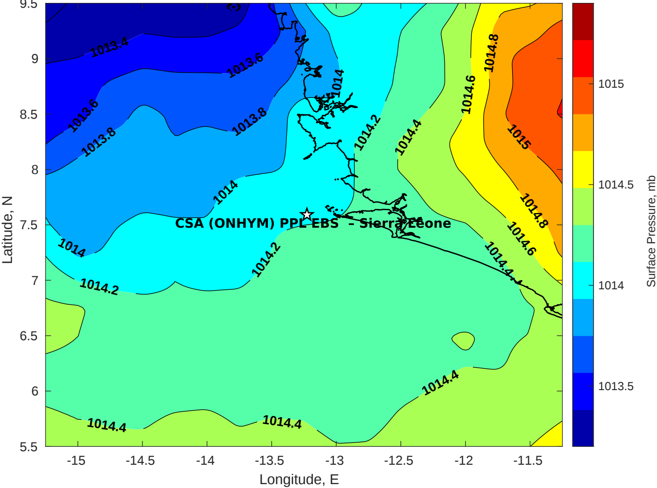
Surface Pressure (mb) for CSA (ONHYM) PPL EBS - Sierra Leone at 06-Sep-2025 00:00:00
