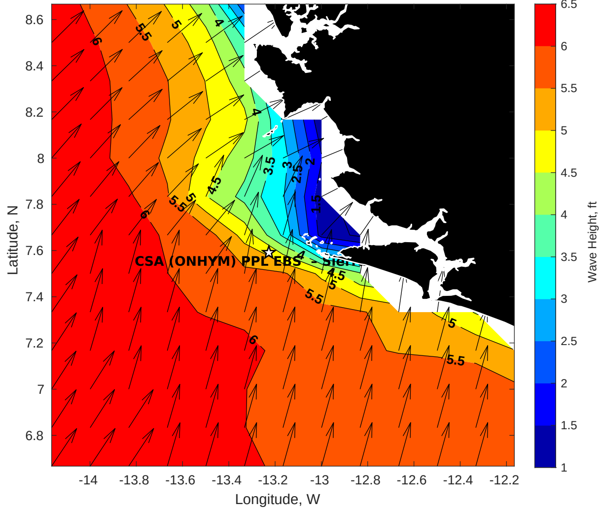
Wave Height (ft) for CSA (ONHYM) PPL EBS - Sierra Leone at 05-Sep-2025 09:00:00
