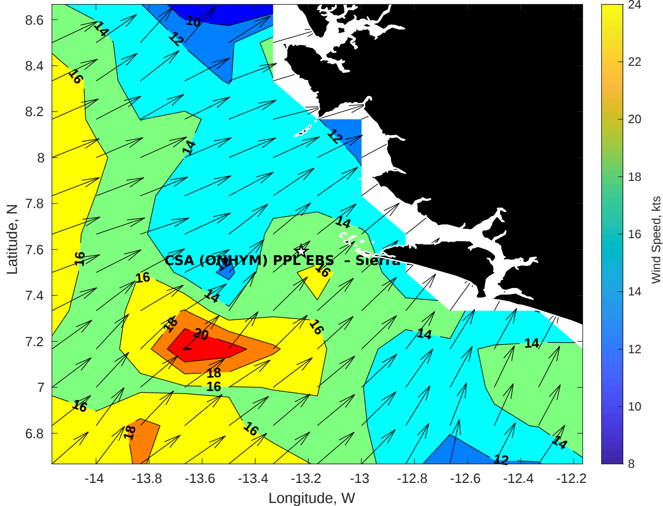
Winds (kts) for CSA (ONHYM) PPL EBS - Sierra Leone at 05-Sep-2025 09:00:00
