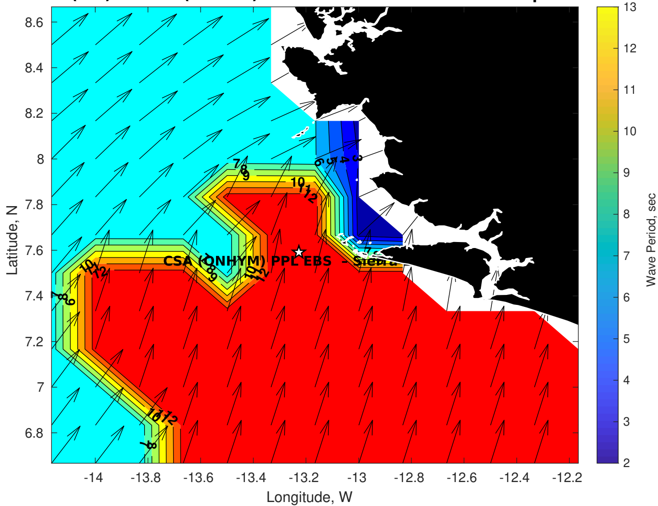
Wave Period (sec) for CSA (ONHYM) PPL EBS - Sierra Leone at 05-Sep-2025 09:00:00
