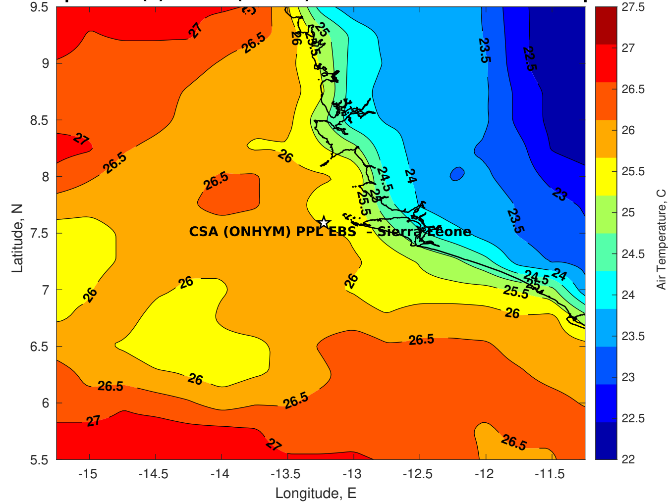
Air Temperature (C) for CSA (ONHYM) PPL EBS - Sierra Leone at 05-Sep-2025
