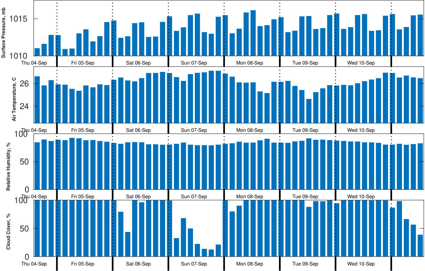
Met Forecast for CSA (ONHYM) PPL EBS - Sierra Leone from 04-Sep-2025 12:00:00 to 11-Sep-2025 12:00:00
