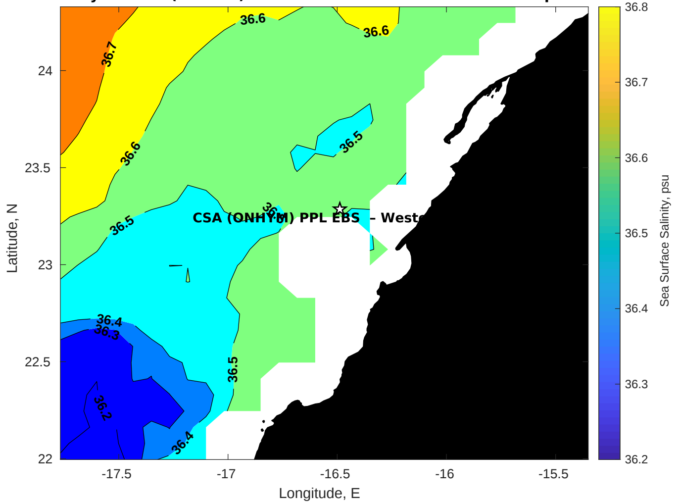
Surface Salinity for CSA (ONHYM) PPL EBS - Western Sahara at 04-Sep-2025 00:00:00
