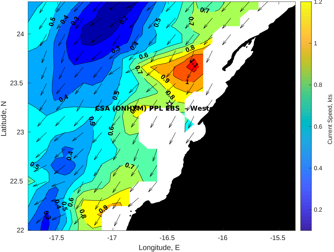
Surface Currents for CSA (ONHYM) PPL EBS - Western Sahara at 04-Sep-2025 00:00:00
