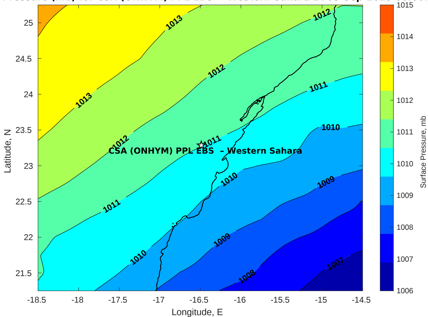
Surface Pressure (mb) for CSA (ONHYM) PPL EBS - Western Sahara at 05-Sep-2025 00:00:00
