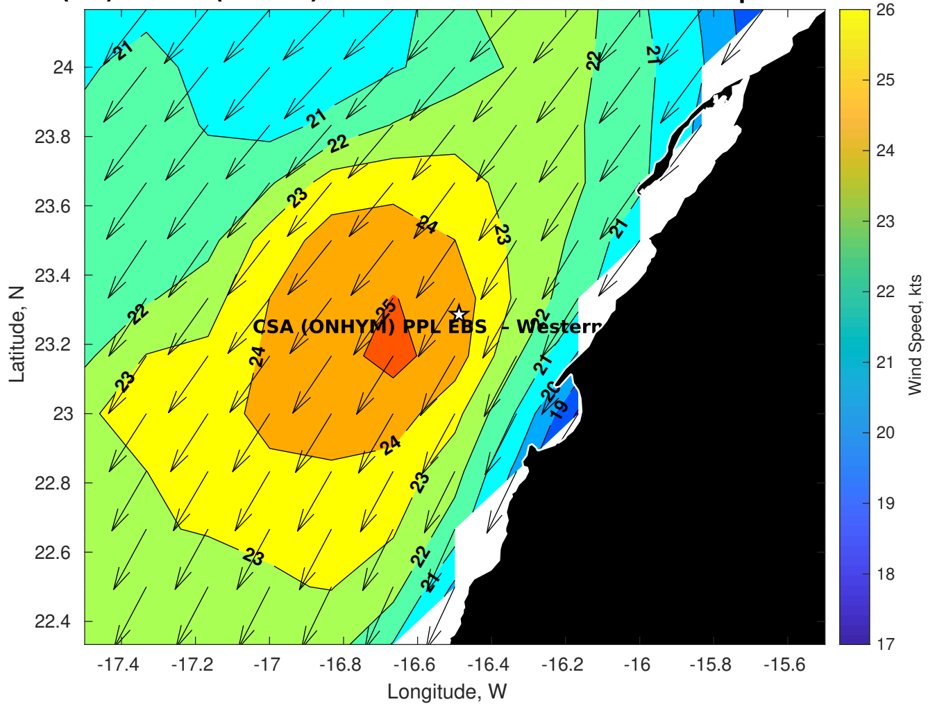
Winds (kts) for CSA (ONHYM) PPL EBS - Western Sahara at 05-Sep-2025 09:00:00
