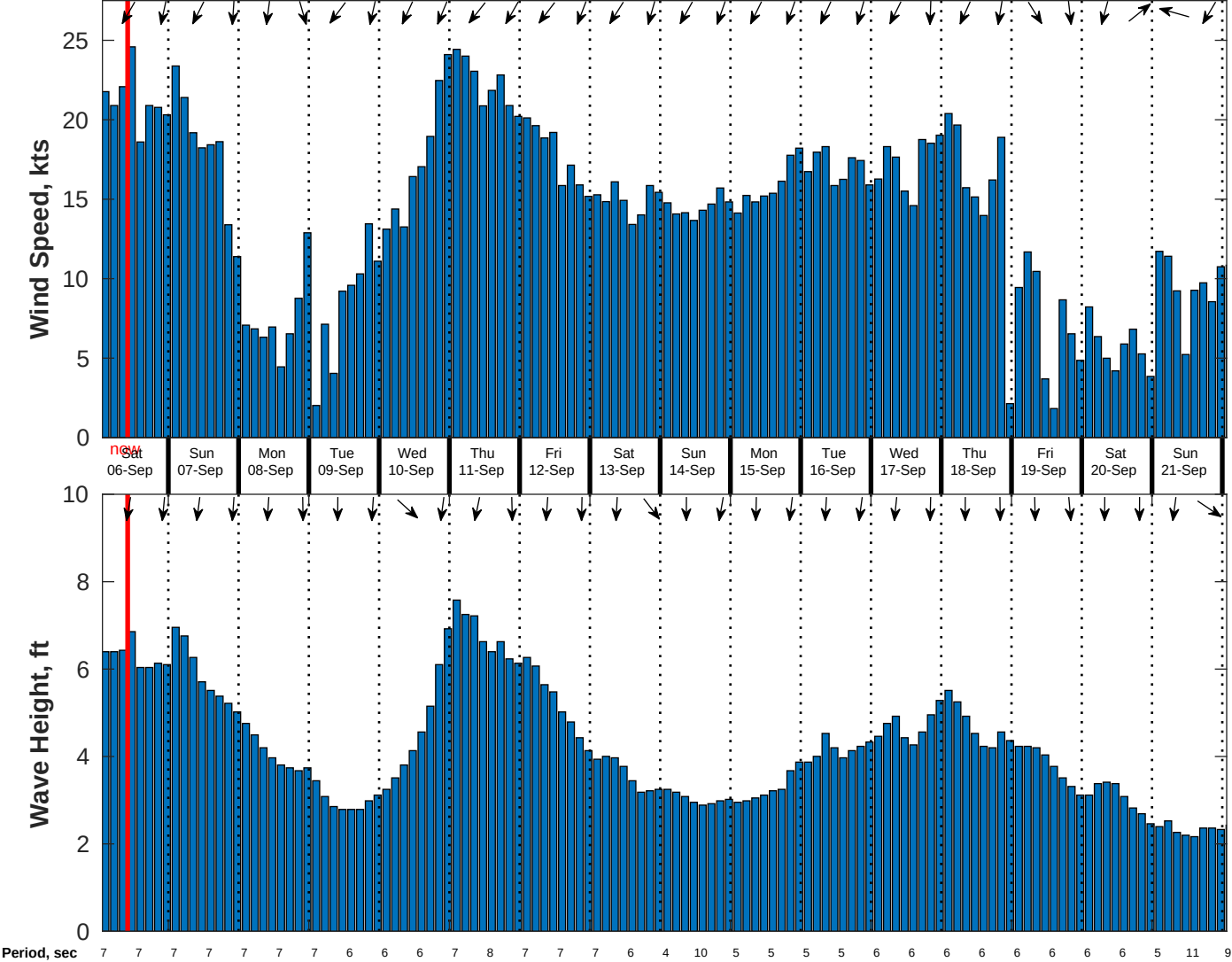
Wind & Wave Forecast for CSA (ONHYM) PPL EBS - Western Sahara from 05-Sep-2025 01:00:00 to 21-Sep-2025 01:00:00
