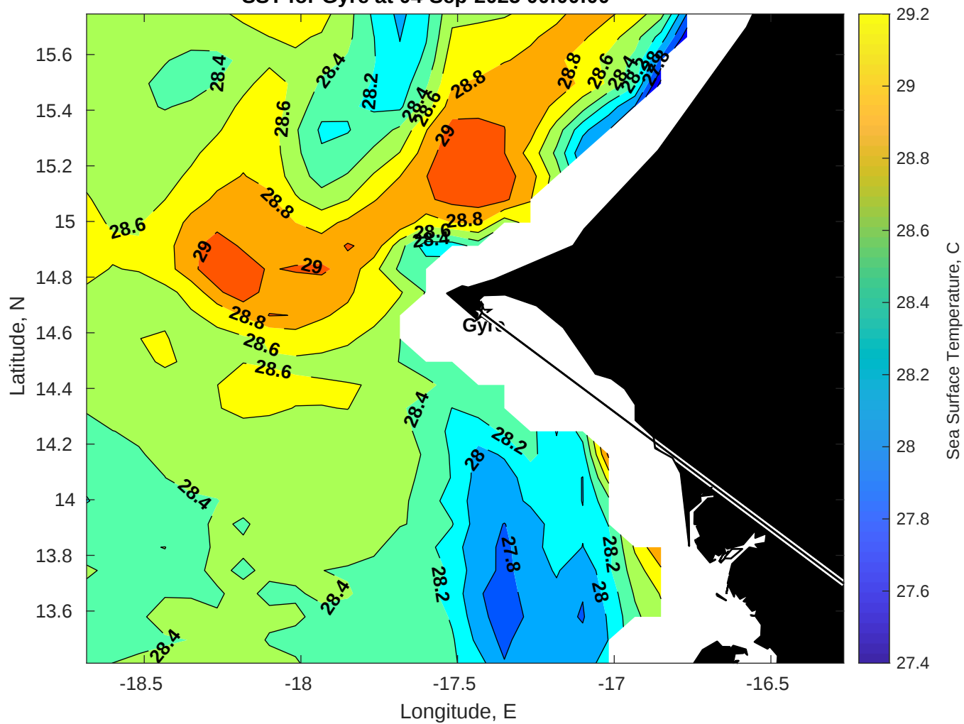
SST for Gyre at 04-Sep-2025 00:00:00
