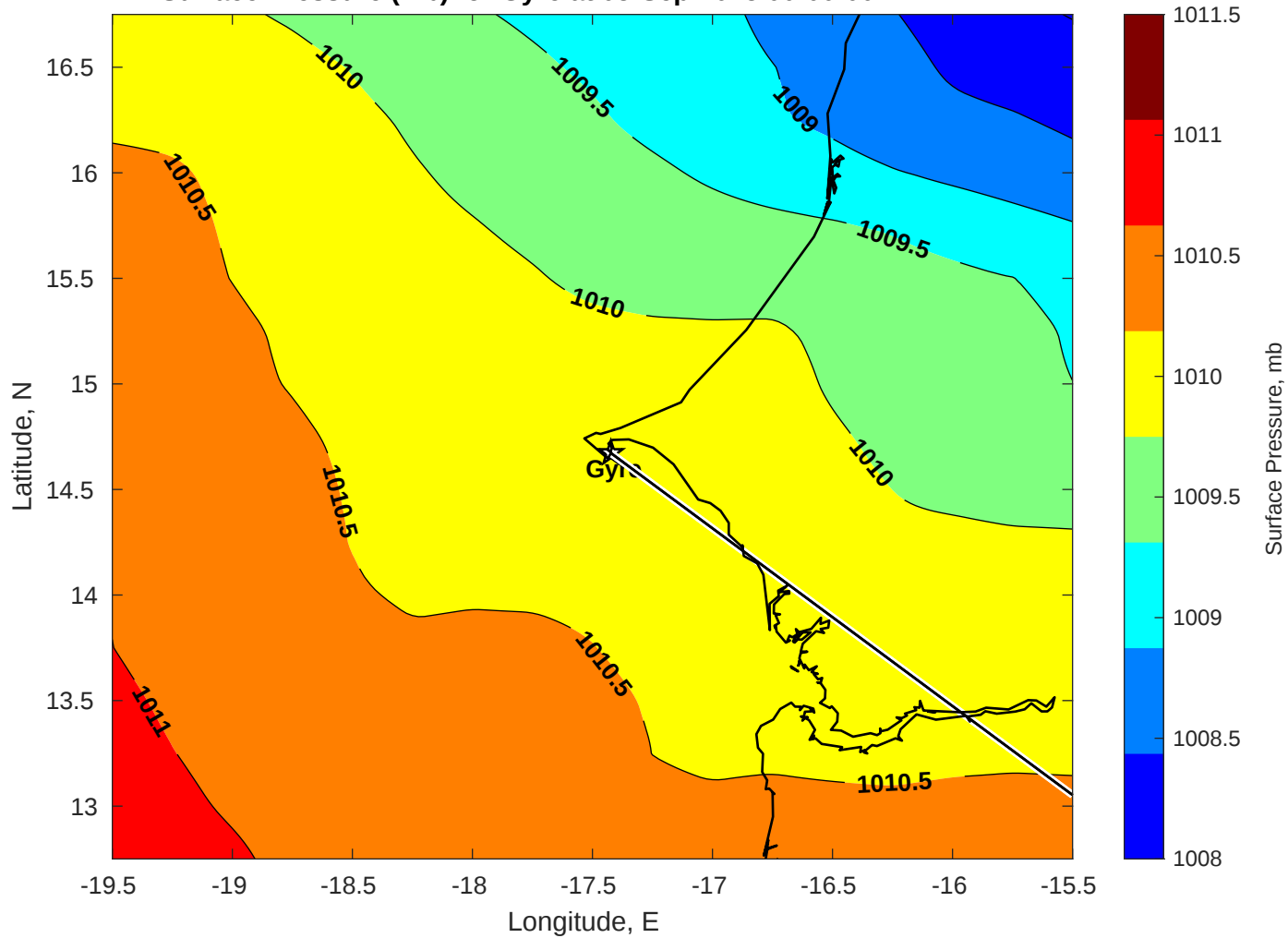
Surface Pressure (mb) for Gyre at 05-Sep-2025 00:00:00
