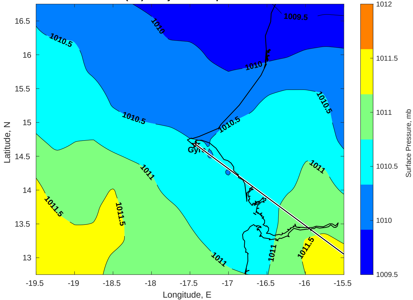
Surface Pressure (mb) for Gyre at 06-Sep-2025 00:00:00
