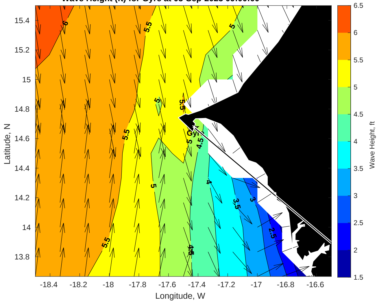
Wave Height (ft) for Gyre at 05-Sep-2025 09:00:00
