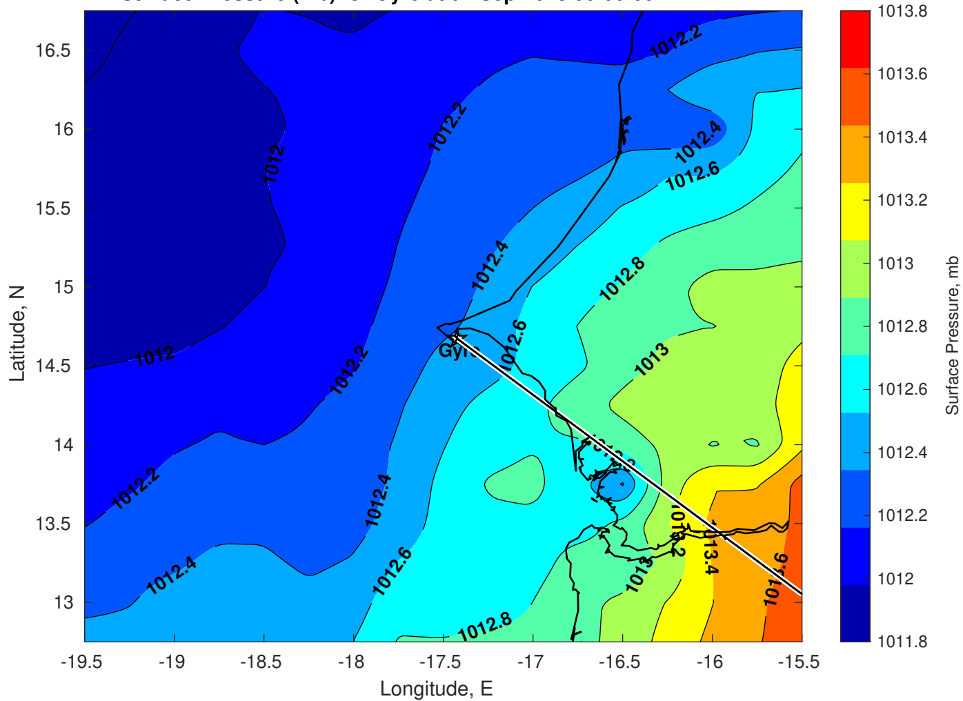
Surface Pressure (mb) for Gyre at 07-Sep-2025 00:00:00
