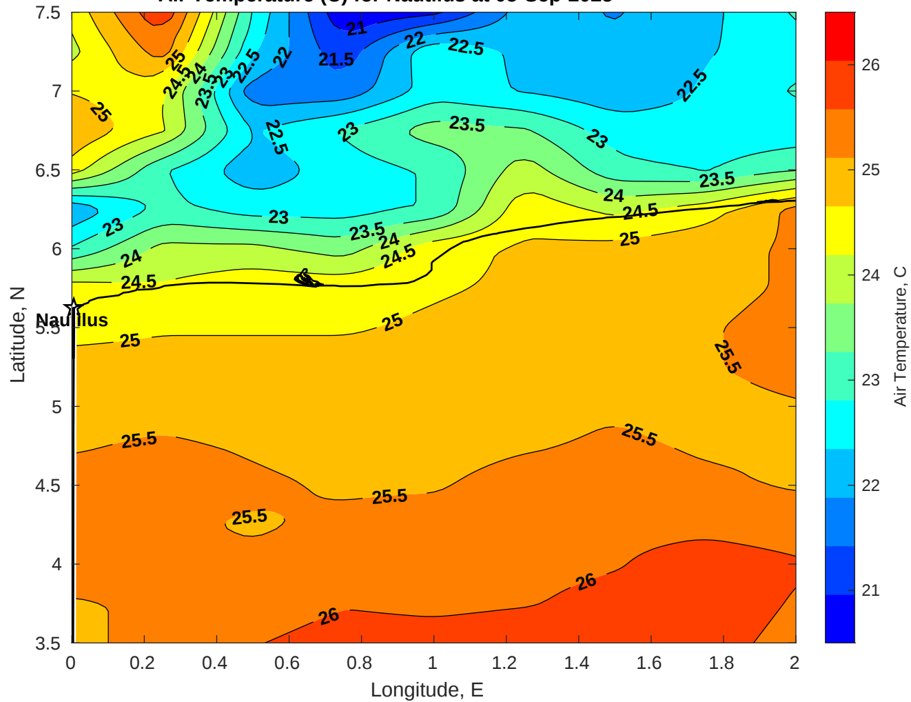
Air Temperature (C) for Nautilus at 05-Sep-2025
