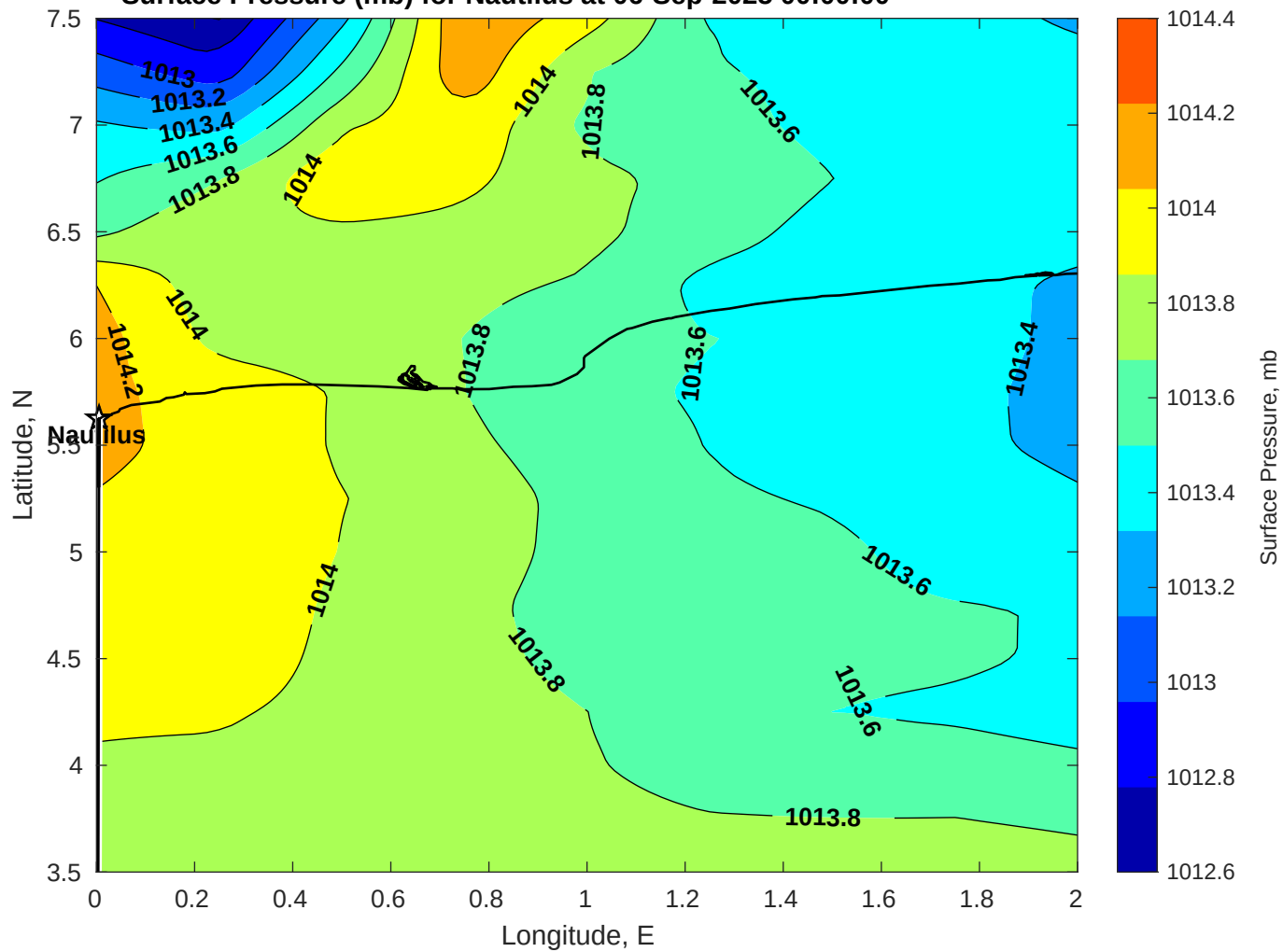
Surface Pressure (mb) for Nautilus at 06-Sep-2025 00:00:00
