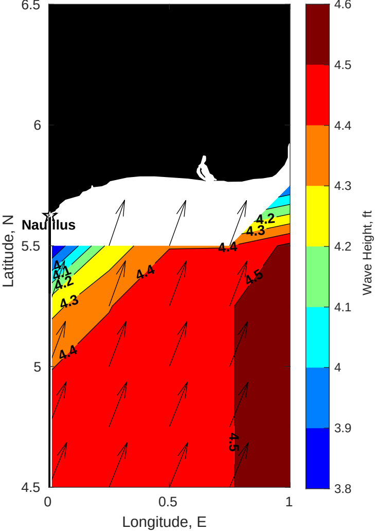
Wave Height (ft) for Nautilus at 05-Sep-2025 09:00:00
