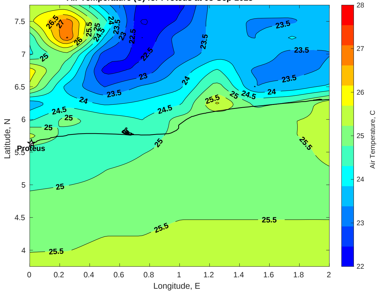
Air Temperature (C) for Proteus at 05-Sep-2025
