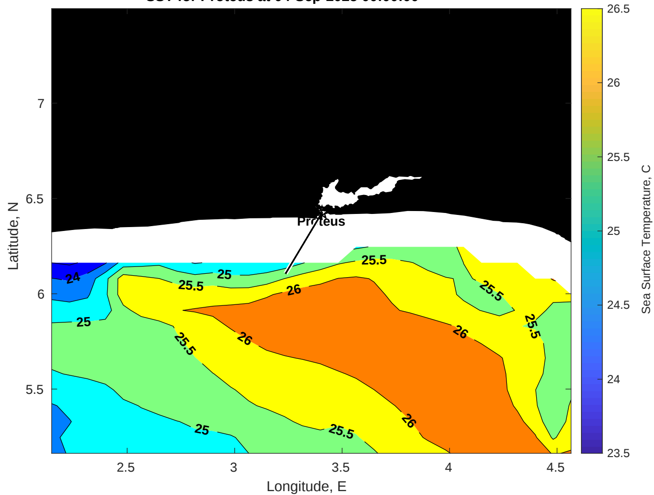
SST for Proteus at 04-Sep-2025 00:00:00
