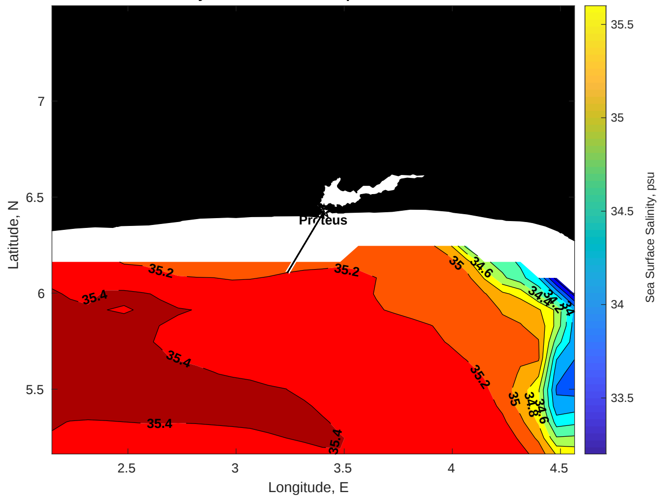
Surface Salinity for Proteus at 04-Sep-2025 00:00:00
