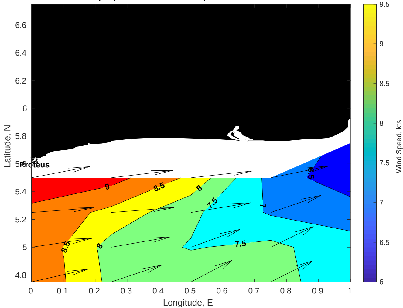
Winds (kts) for Proteus at 05-Sep-2025 09:00:00
