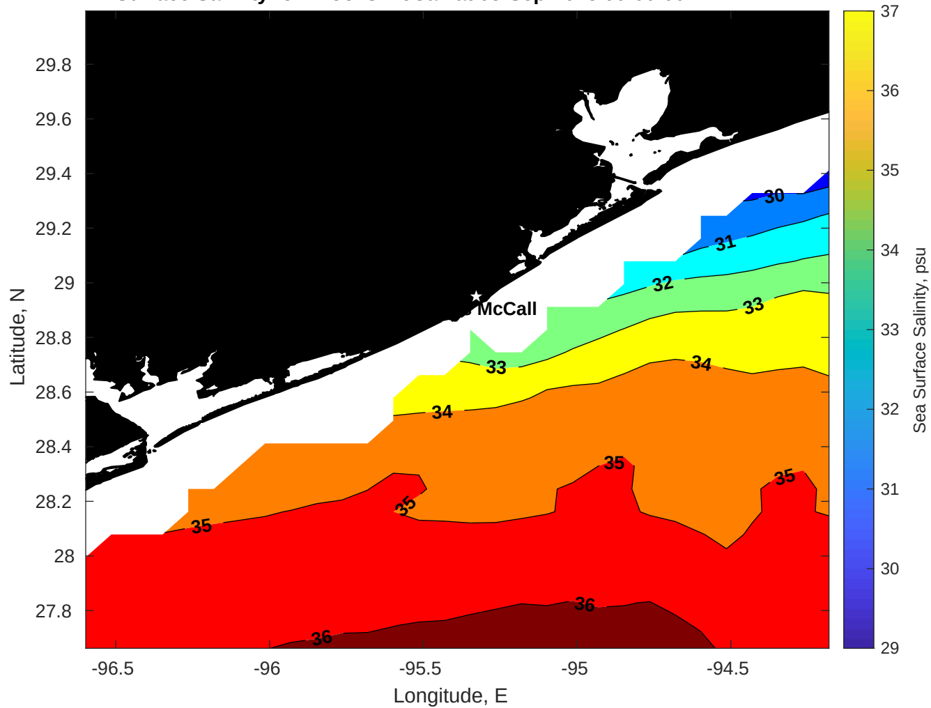
Surface Salinity for Brooks McCall at 05-Sep-2025 00:00:00
