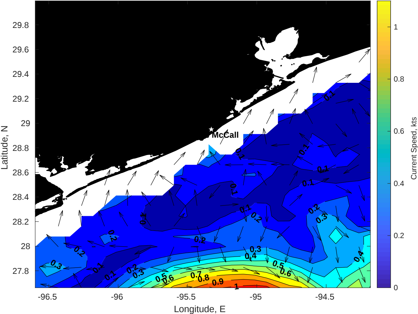
Surface Currents for Brooks McCall at 05-Sep-2025 00:00:00
