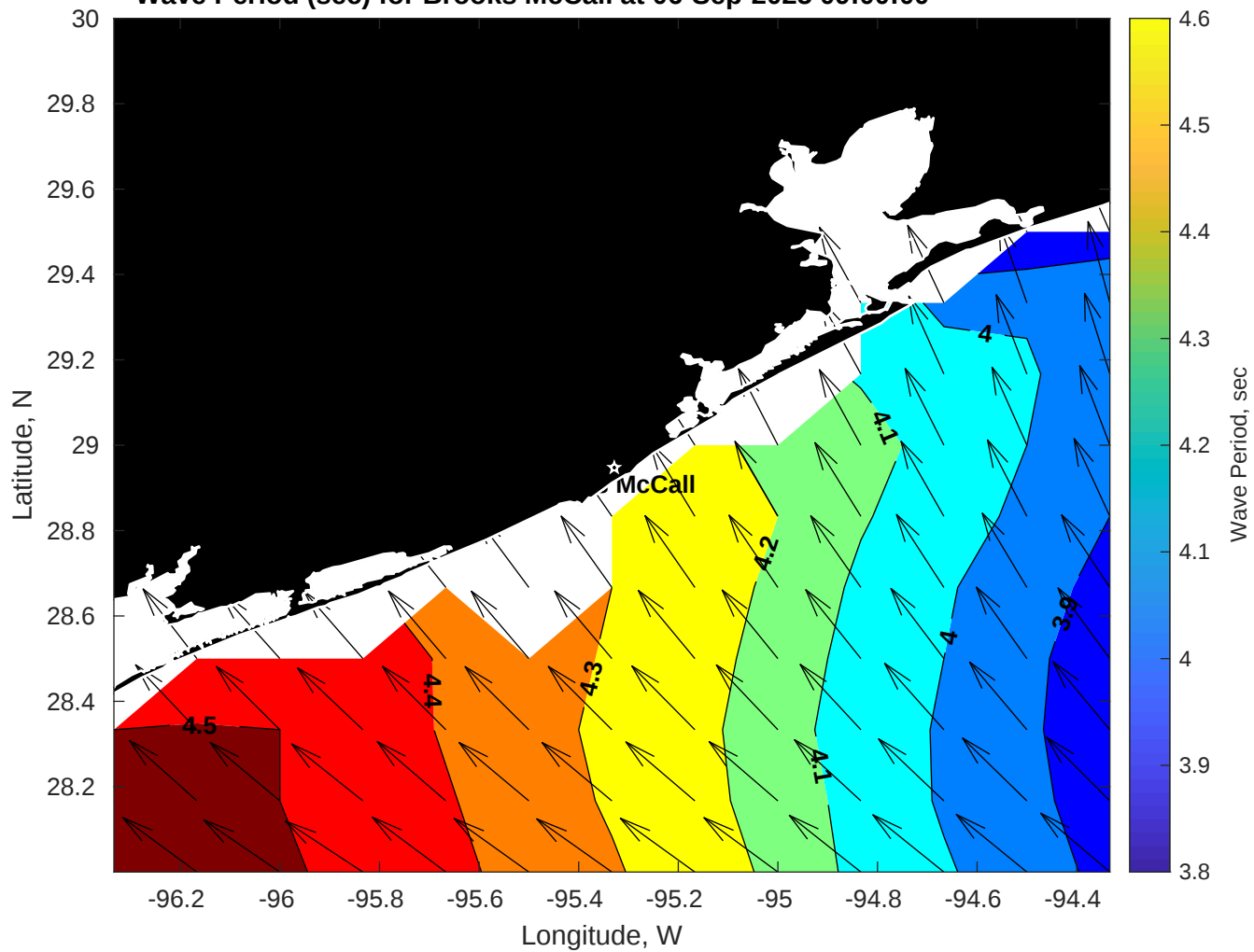
Wave Period (sec) for Brooks McCall at 06-Sep-2025 09:00:00
