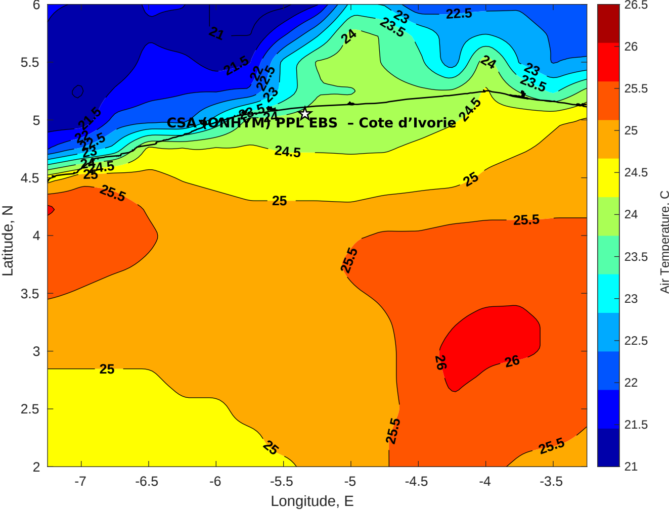
Air Temperature (C) for CSA (ONHYM) PPL EBS - Cote d'Ivoire at 06-Sep-2025
