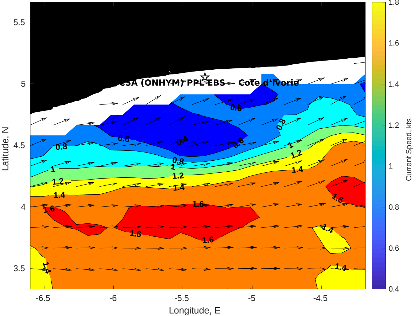
Surface Currents for CSA (ONHYM) PPL EBS - Cote d'Ivoire at 05-Sep-2025 00:00:00
