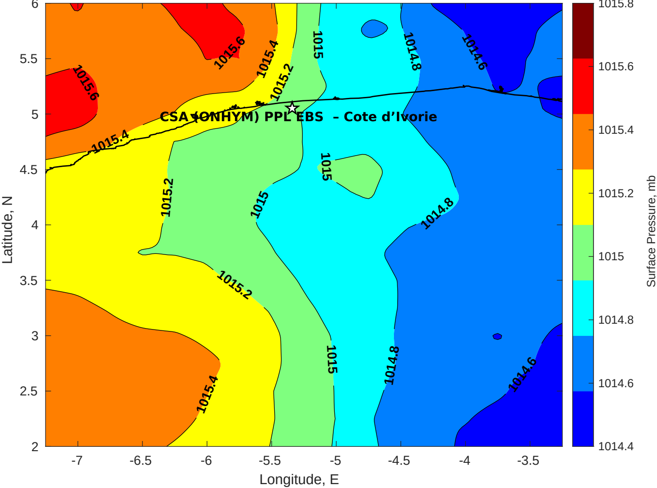
Surface Pressure (mb) for CSA (ONHYM) PPL EBS - Cote d'Ivoire at 06-Sep-2025 00:00:00
