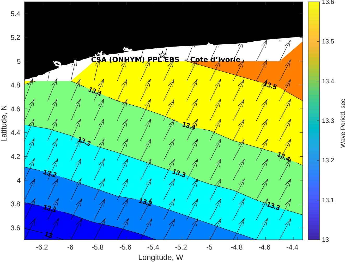
Wave Period (sec) for CSA (ONHYM) PPL EBS - Cote d'Ivoire at 06-Sep-2025 09:00:00
