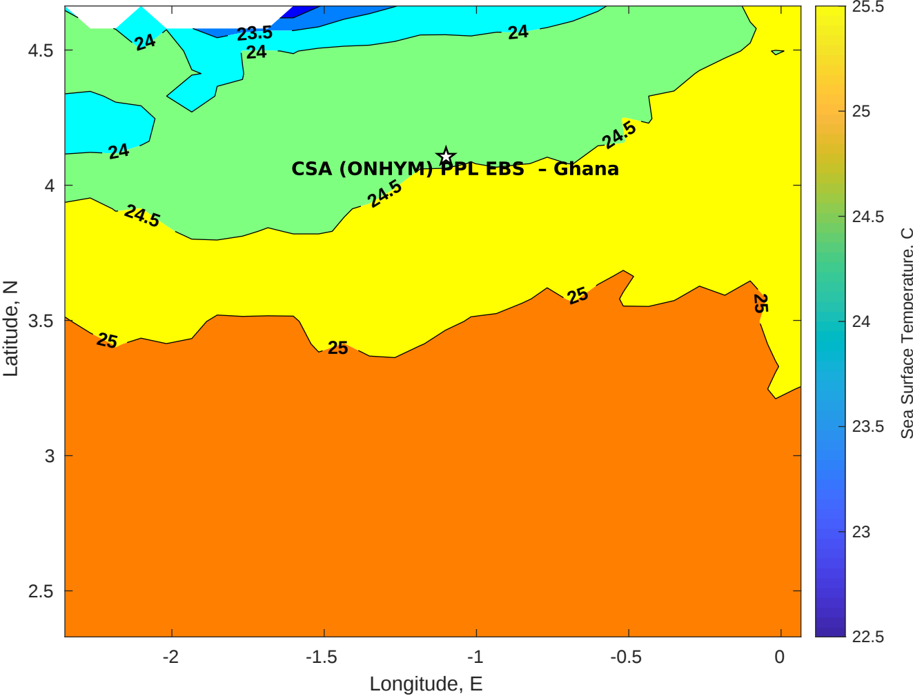
SST for CSA (ONHYM) PPL EBS - Ghana at 05-Sep-2025 00:00:00
