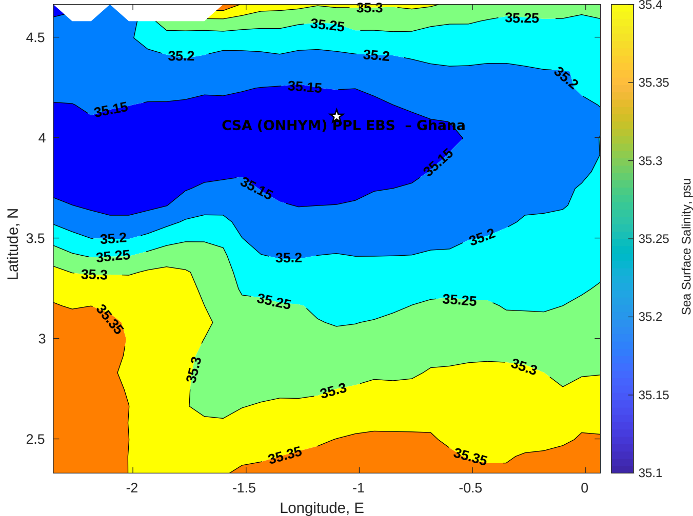
Surface Salinity for CSA (ONHYM) PPL EBS - Ghana at 05-Sep-2025 00:00:00
