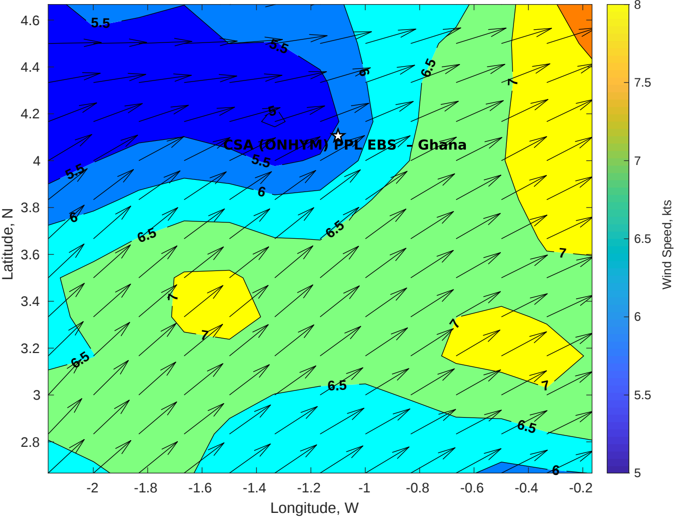
Winds (kts) for CSA (ONHYM) PPL EBS - Ghana at 06-Sep-2025 09:00:00
