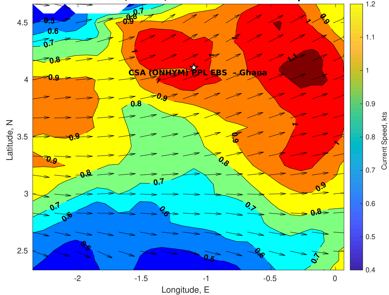
Surface Currents for CSA (ONHYM) PPL EBS - Ghana at 05-Sep-2025 00:00:00
