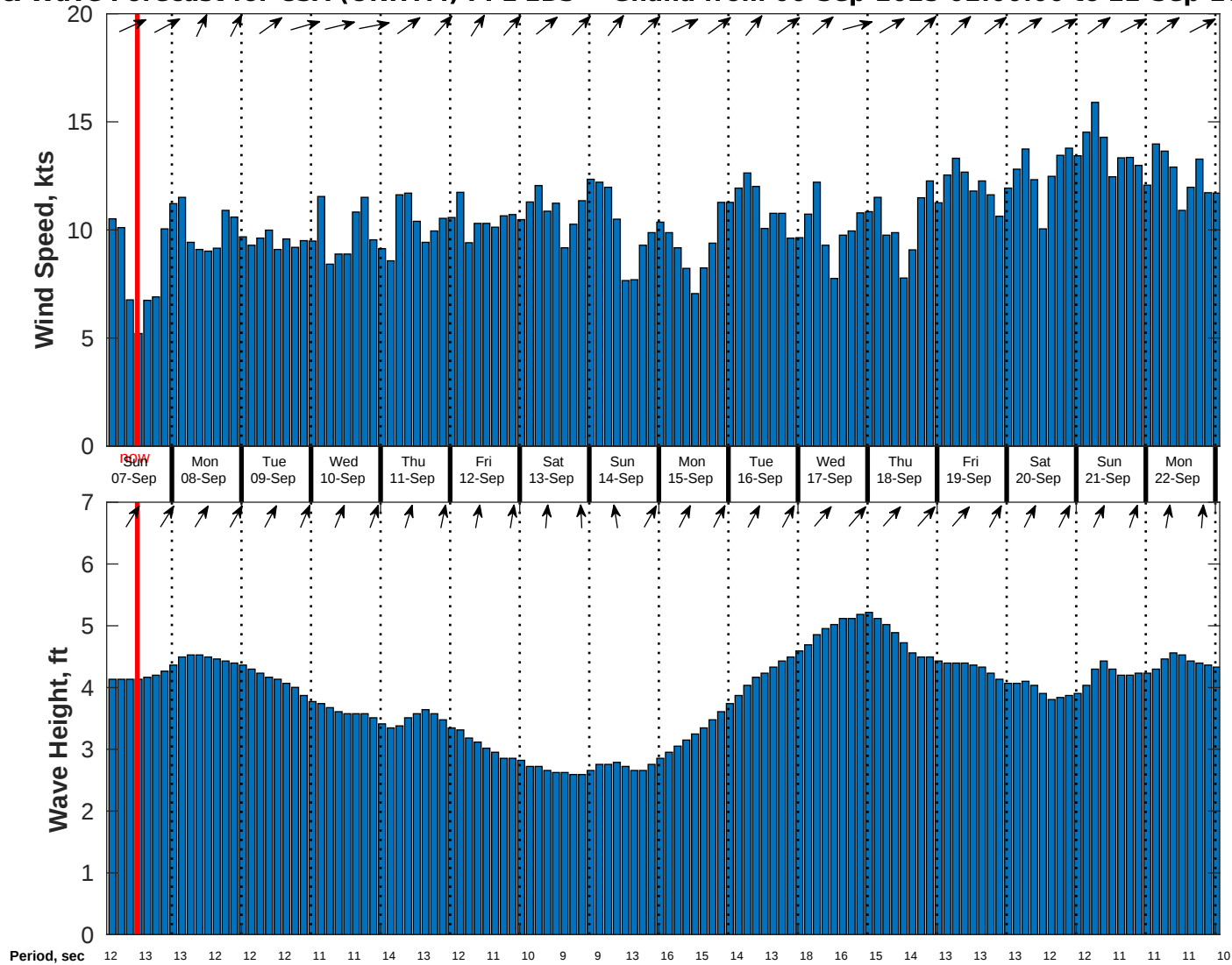
Wind & Wave Forecast for CSA (ONHYM) PPL EBS - Ghana from 06-Sep-2025 02:00:00 to 22-Sep-2025 02:00:00
