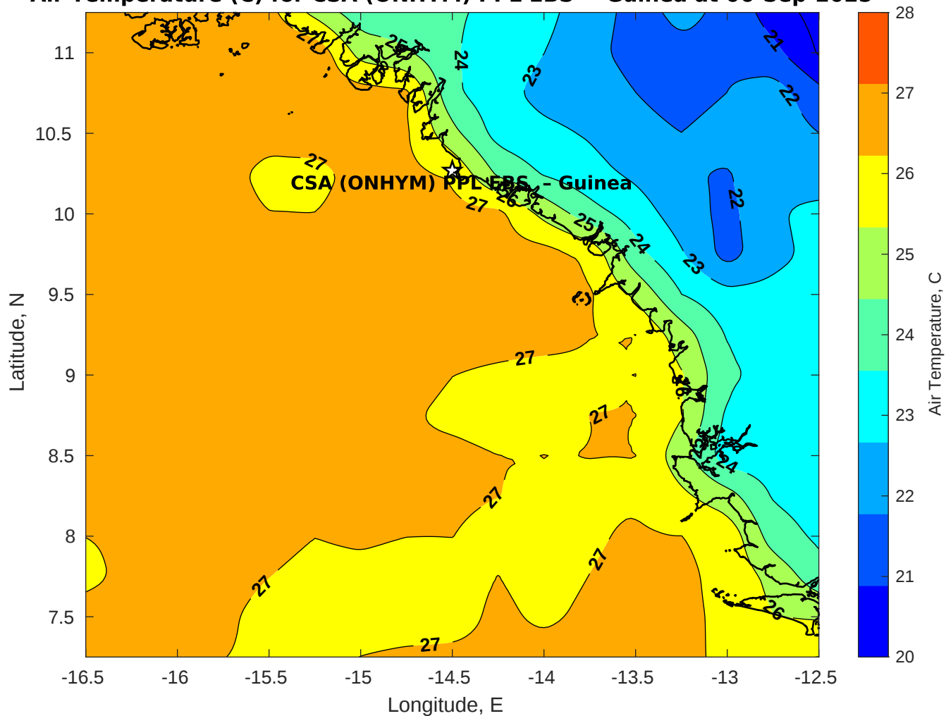
Air Temperature (C) for CSA (ONHYM) PPL EBS - Guinea at 06-Sep-2025
