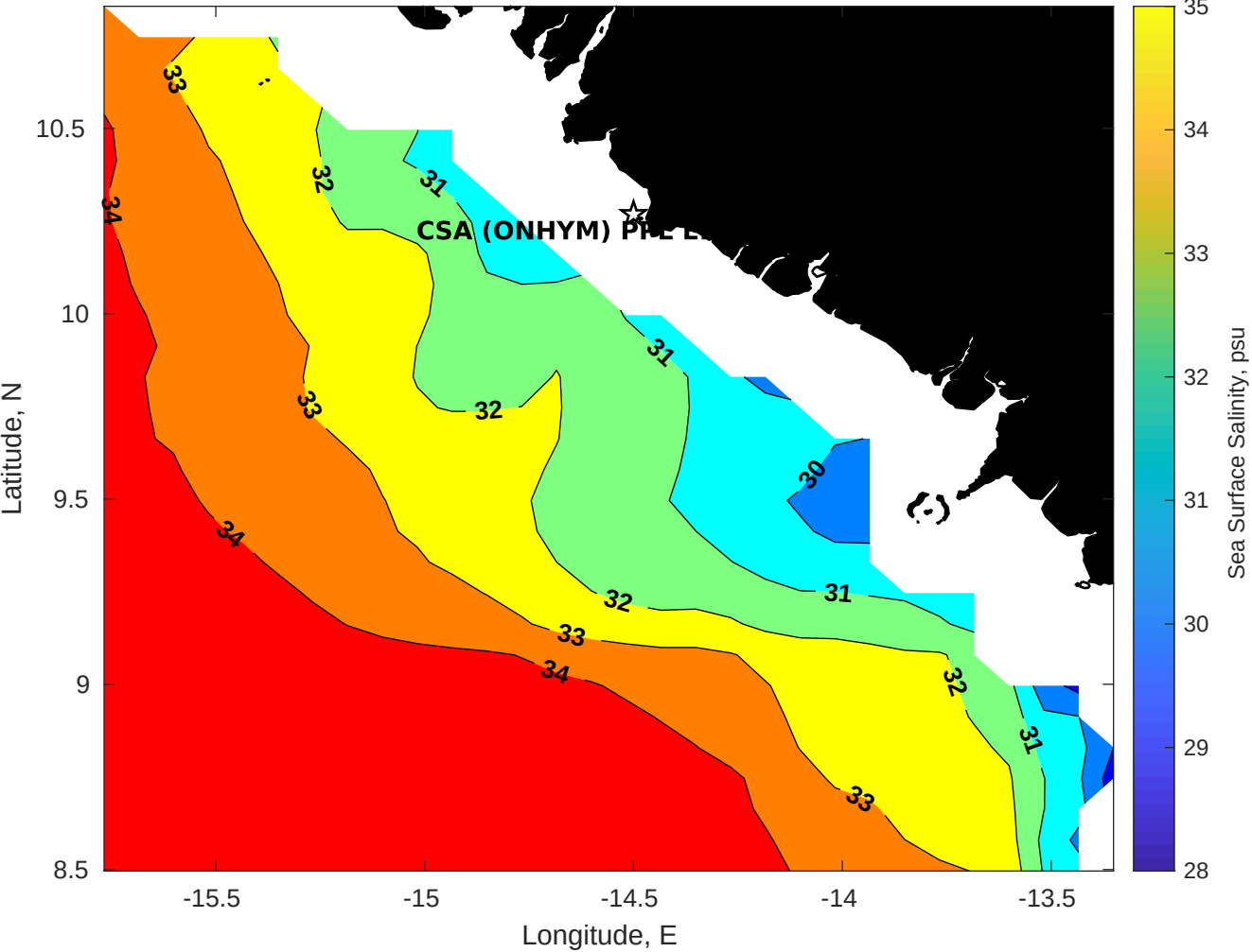
Surface Salinity for CSA (ONHYM) PPL EBS - Guinea at 05-Sep-2025 00:00:00
