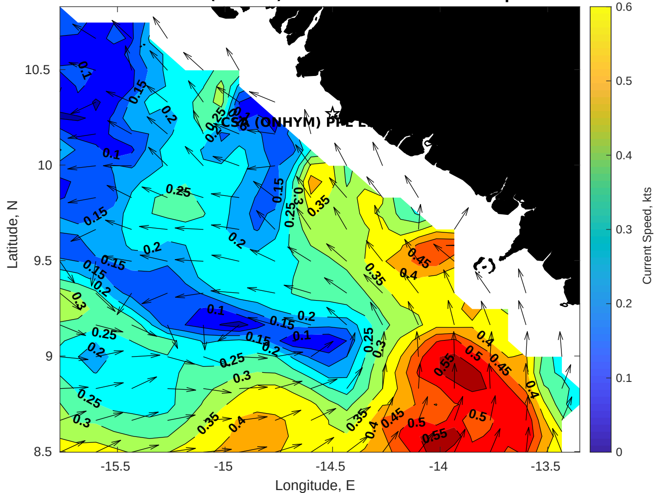
Surface Currents for CSA (ONHYM) PPL EBS - Guinea at 05-Sep-2025 00:00:00
