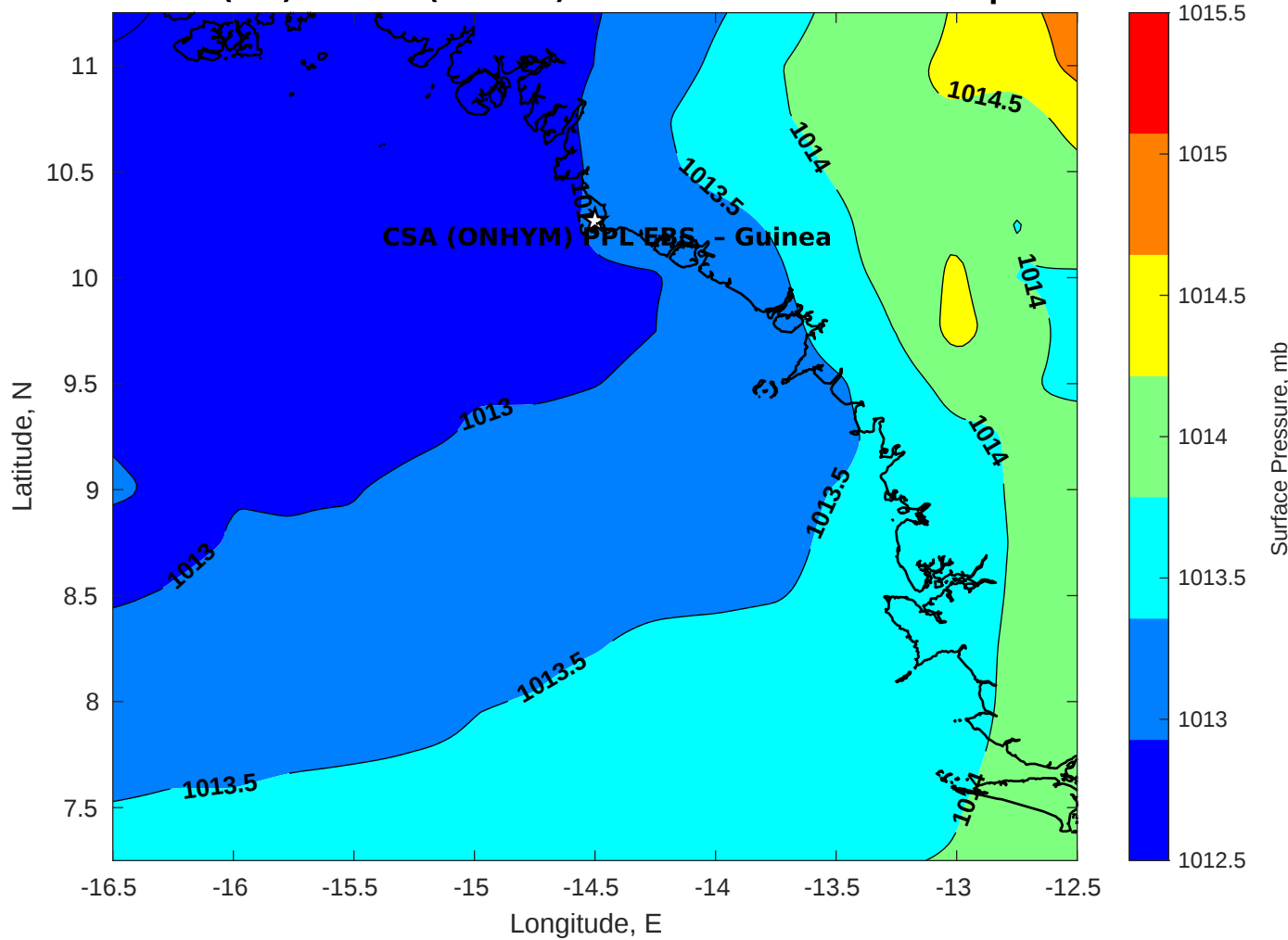
Surface Pressure (mb) for CSA (ONHYM) PPL EBS - Guinea at 06-Sep-2025 00:00:00
