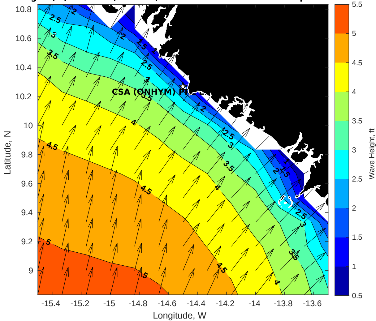
Wave Height (ft) for CSA (ONHYM) PPL EBS - Guinea at 06-Sep-2025 09:00:00
