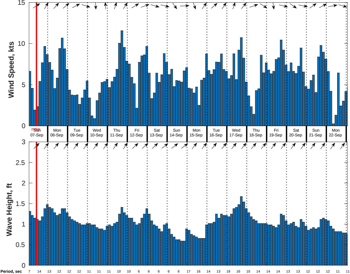
Wind & Wave Forecast for CSA (ONHYM) PPL EBS - Guinea from 06-Sep-2025 01:00:00 to 22-Sep-2025 01:00:00
