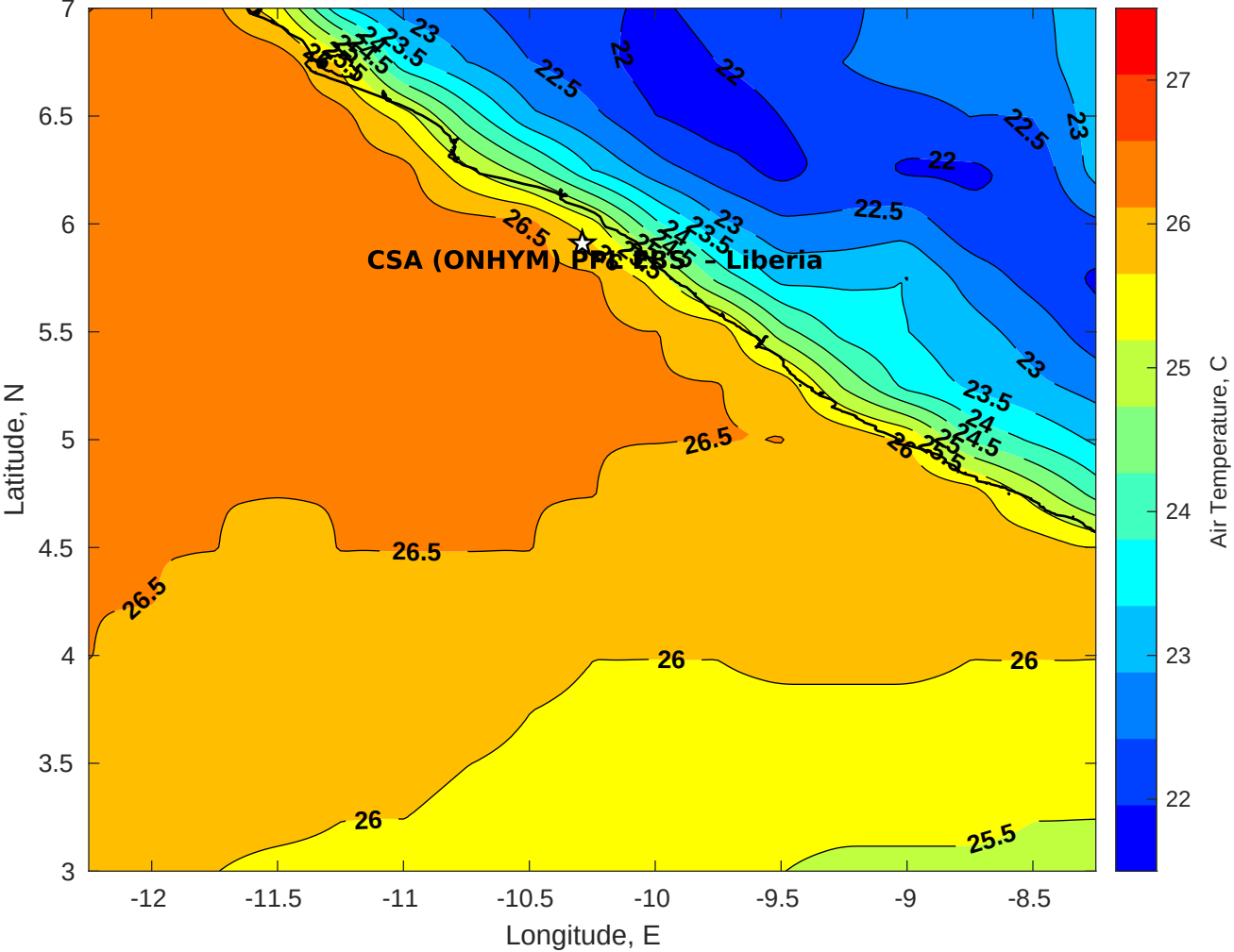
Air Temperature (C) for CSA (ONHYM) PPL EBS - Liberia at 06-Sep-2025
