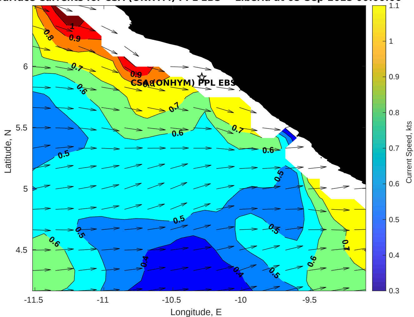
Surface Currents for CSA (ONHYM) PPL EBS - Liberia at 05-Sep-2025 00:00:00
